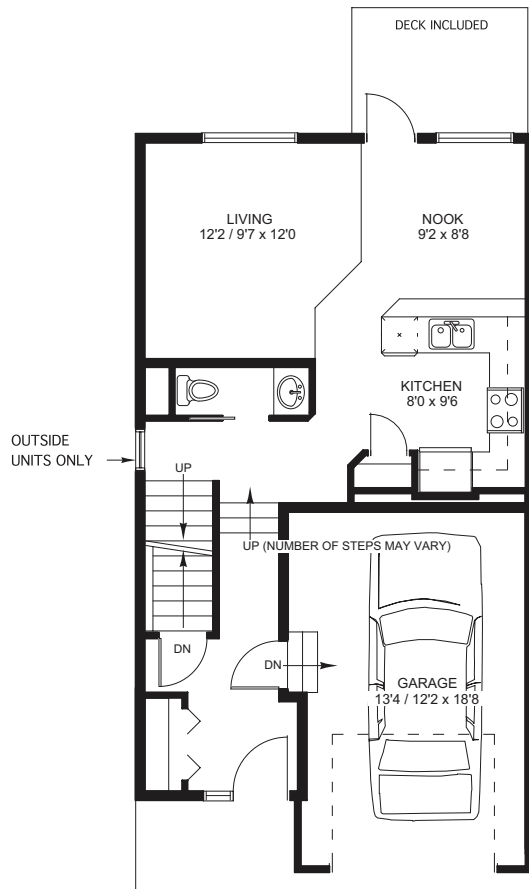
MAIN FLOOR Alternate 1 602 sq. ft. GARAGE 263/251 sq. ft.
