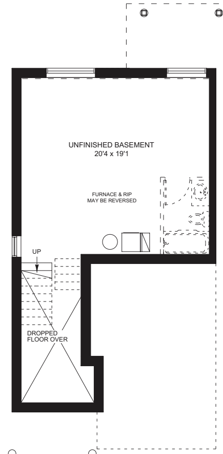
UNDEVELOPED BASEMENT 602 sq. ft.
