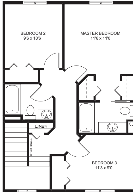
UPPER FLOOR Alternate 5
