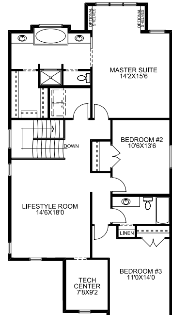
Optional 3-Bedroom Upper Floor
