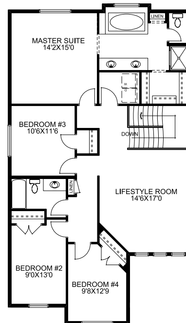
Alternate Upper Floor
